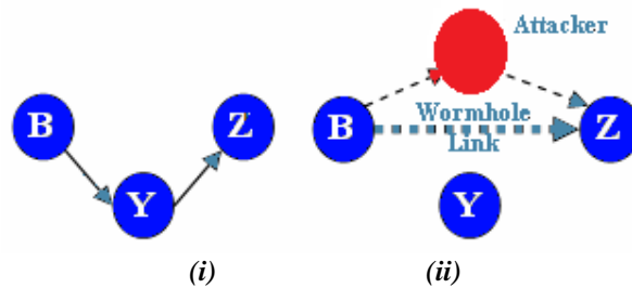
Figure 3: Wormhole Attack
